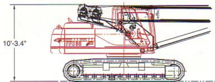
LOW PROFILE CONFIGURATION
