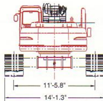
LOW PROFILE CONFIGURATION
